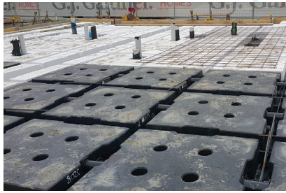
IN-SLAB
